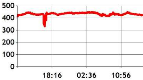
RMS VOLTAGE VARIATION TIME PLOT OF CH1
