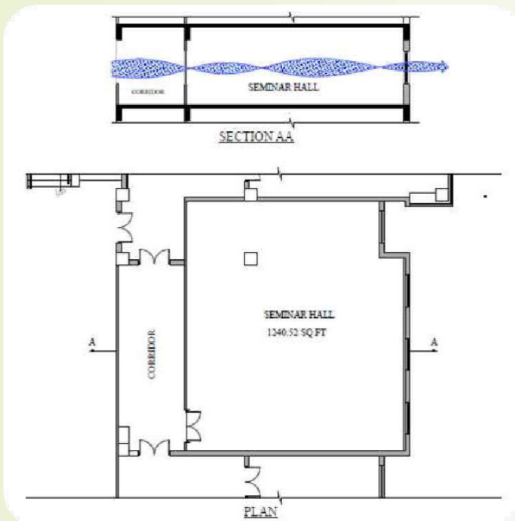
Figure 38 : Typical cross ventilation schematic
